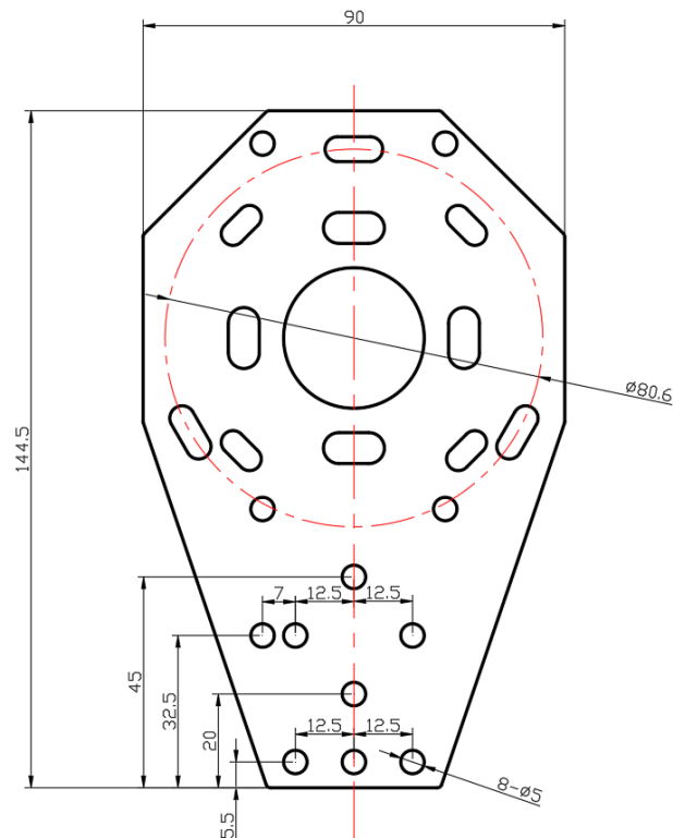
Installation pallet size chart (unit: mm)
